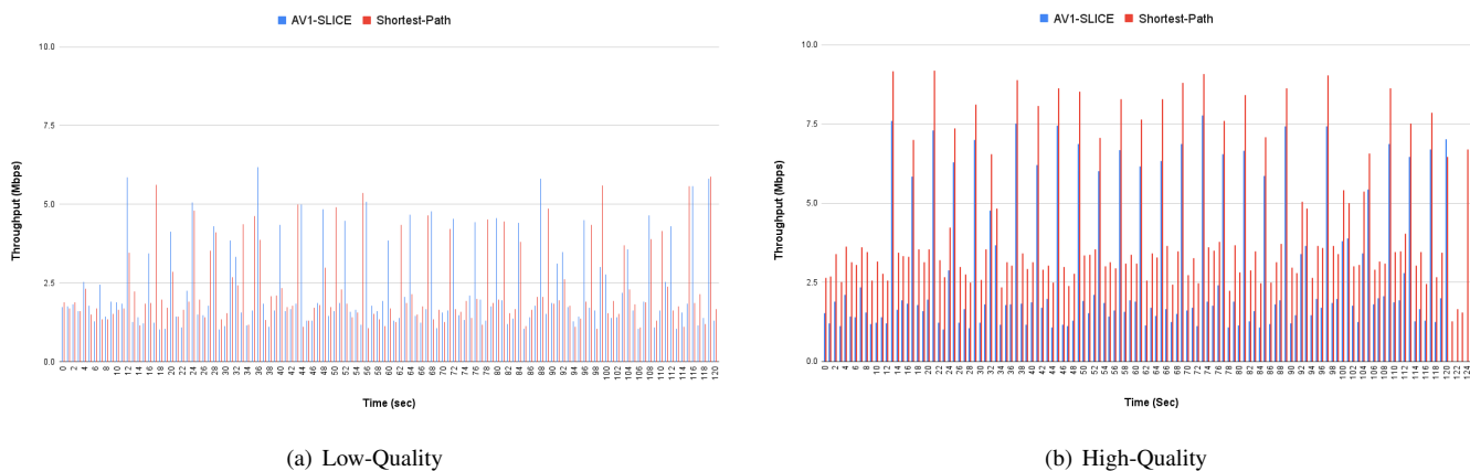
Fig. 2: Throughput - AV1-SLICE vs Shortest Path
